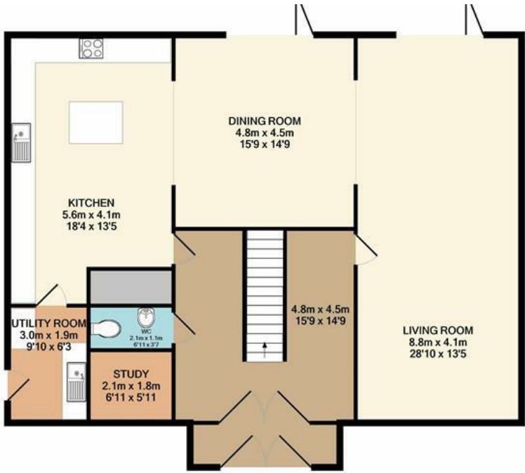
GROUND FLOOR APPROX. FLOOR AREA 126.0 SQ.M. (1356 SQ.FT.)
